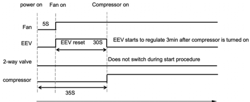
Figure 3 – Power ON logic
